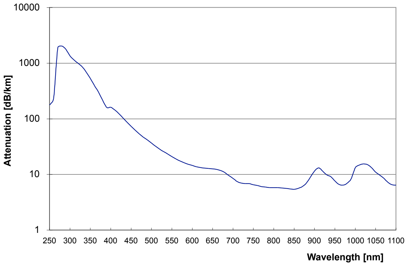
Spectra scan of attenuation for 200um, NA=0.37 H-PCF, HL-20/06**
